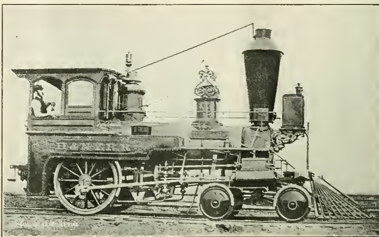
HACKENSACK, BUILT BY ROGERS IN 1860, FOR N. Y. & HACKENSACK BROAD GAUGE, NOW PART OF ERIE.
